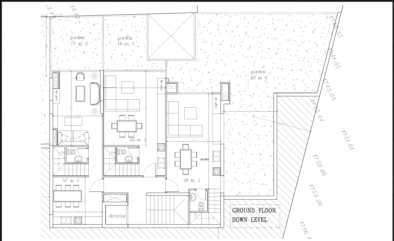
GROUND FLOOR — LIVING LEVEL
