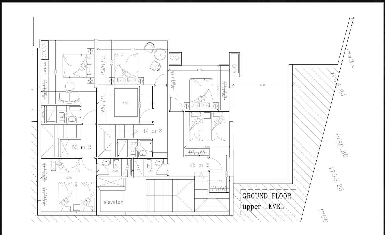
GROUND FLOOR — BEDROOM LEVEL
