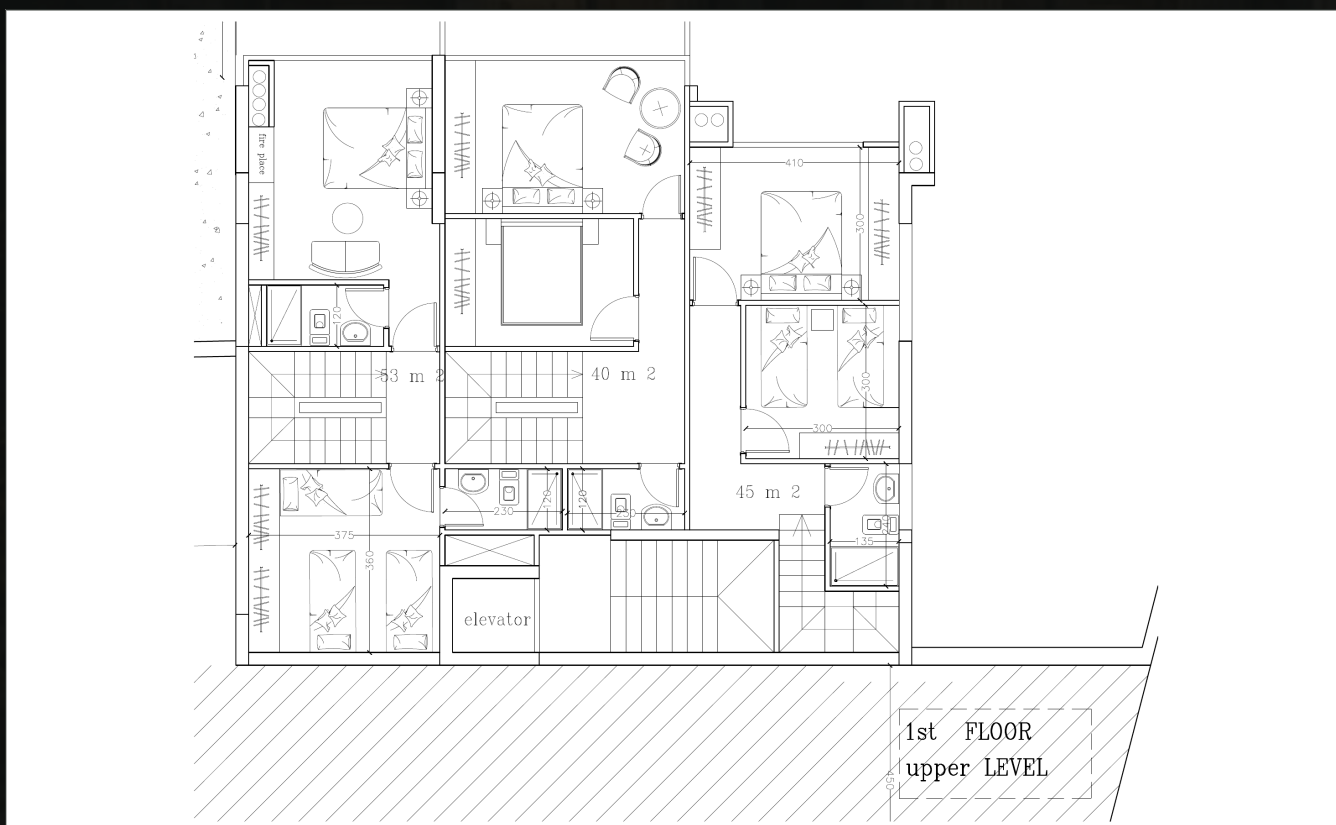
FIRST FLOOR — BEDROOM LEVEL
