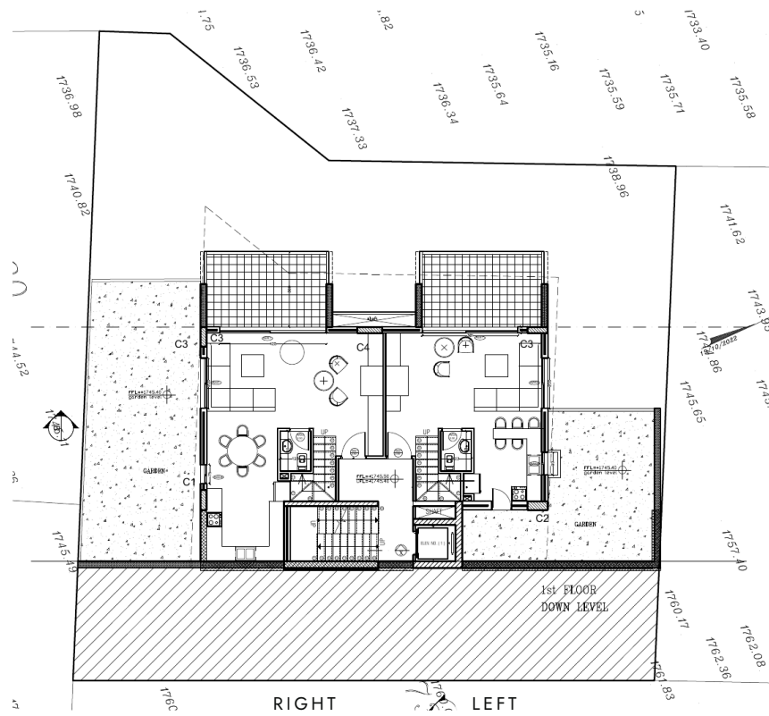
PLAN — FIRST FLOOR, LIVING LEVEL
