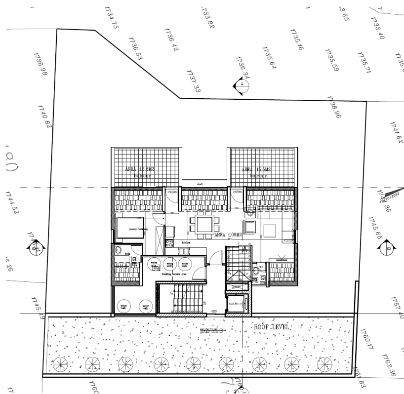
PLAN — ROOF LEVEL, OPTIONAL EXTENSION
