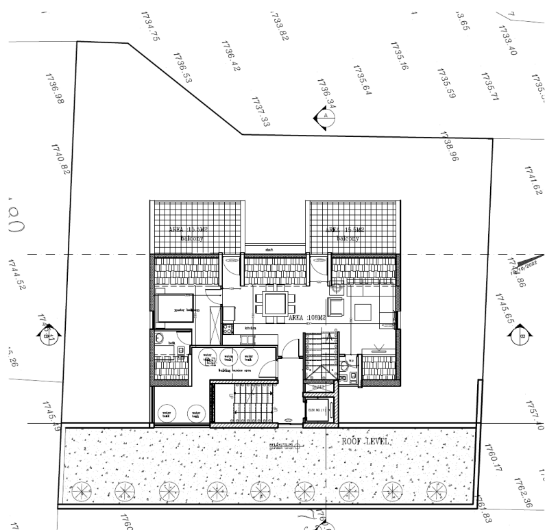
PLAN — ROOF LEVEL, OPTIONAL EXTENSION
