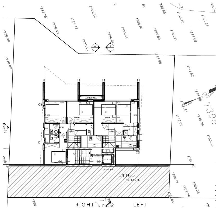
PLAN — FIRST FLOOR, BEDROOM LEVEL
